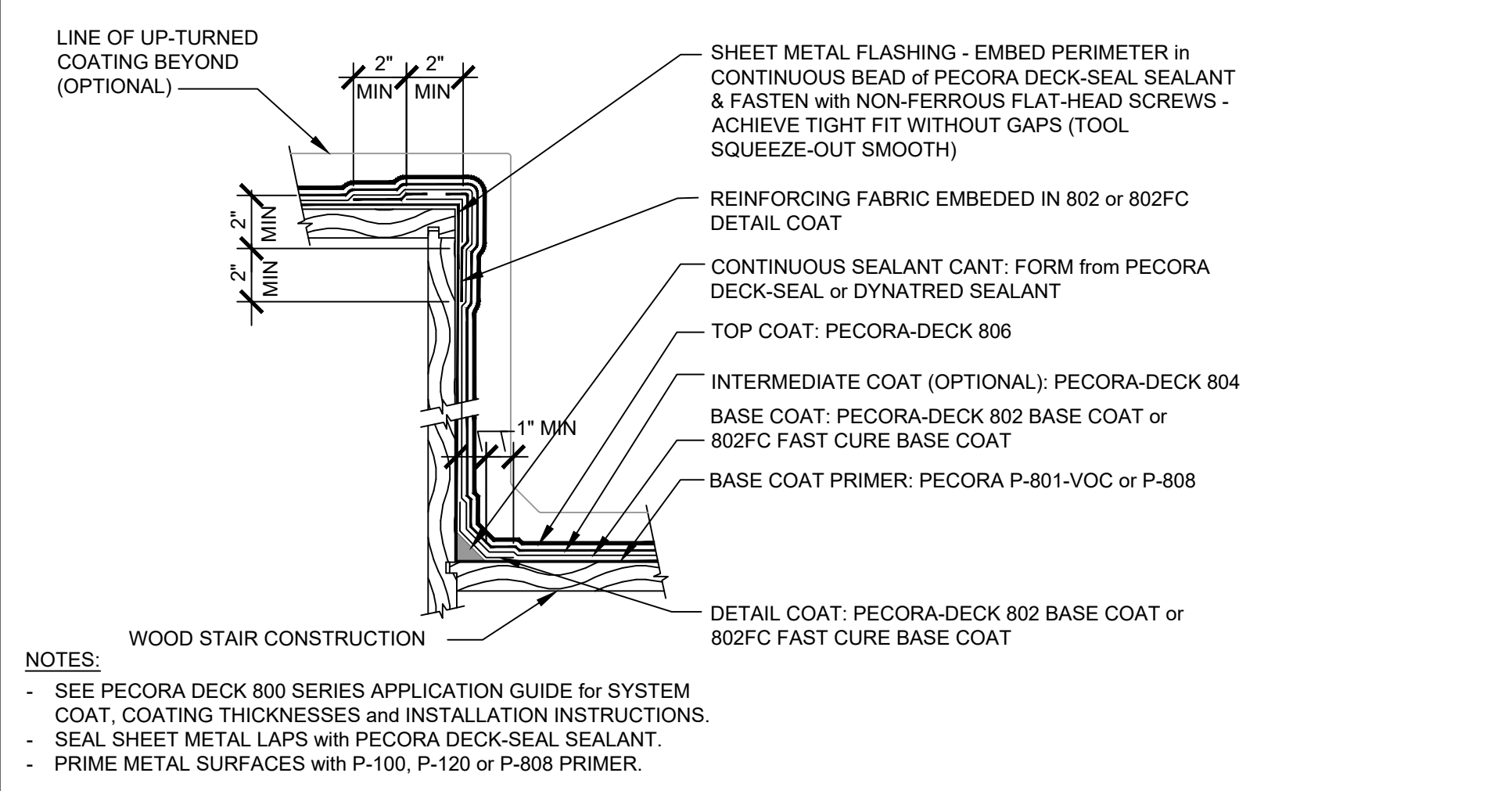
122C: PLYWOOD STAIR TREATMENT
