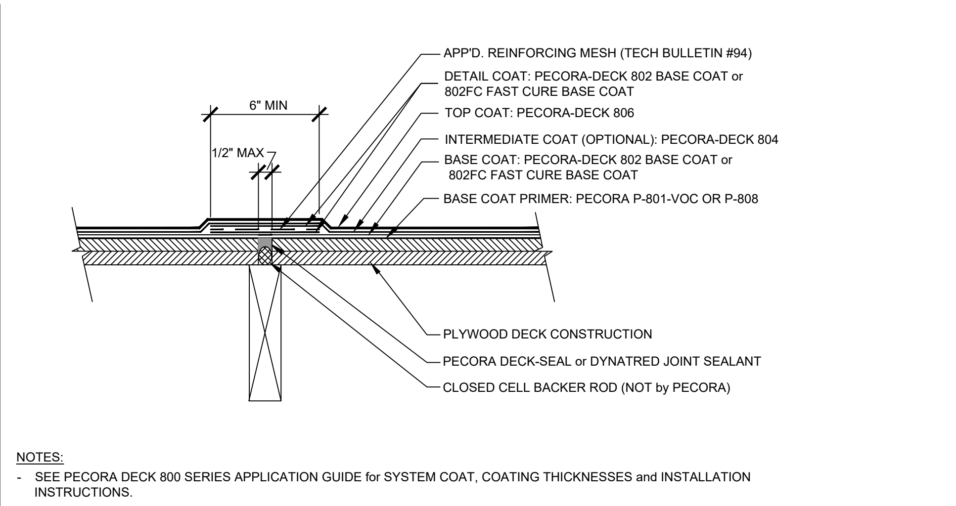
123A: PLYWOOD DECK-TO-DECK JOINT
