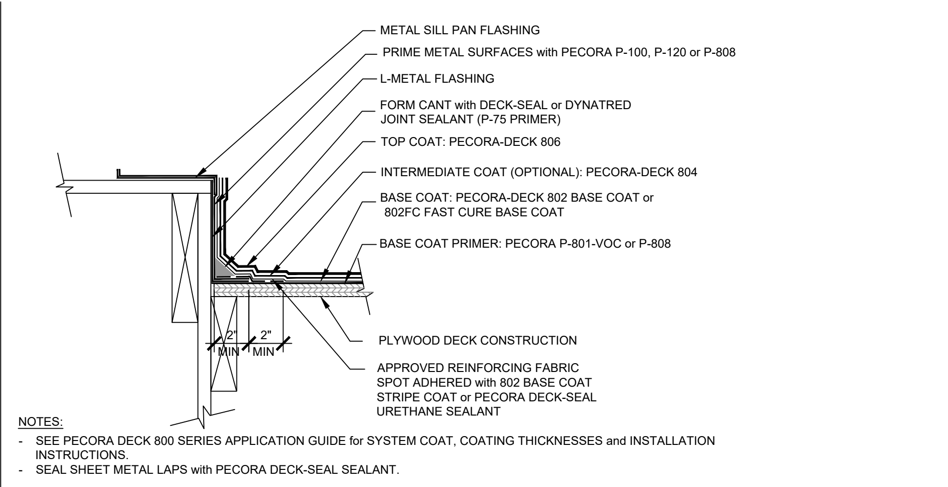
122A: PLYWOOD DECK FLASHING TIE-IN
