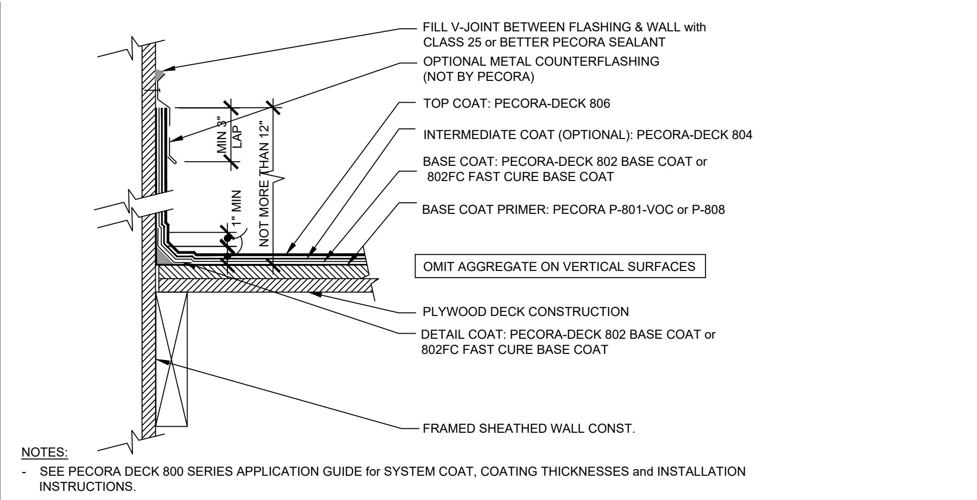
122: PLYWOOD DECK-TO-WALL STATIC JOINT
